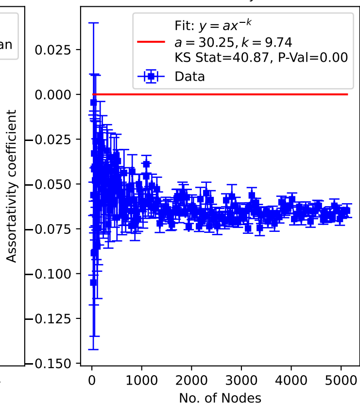
Power Law Fit and Plot of Nodes vs Assortativity coefficient
