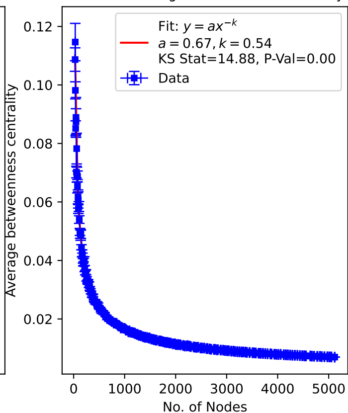
Power Law Fit and Plot of Nodes vs Average betweenness centrality
