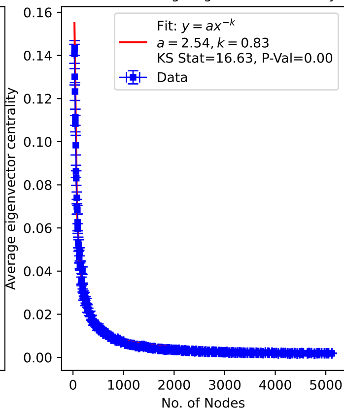
Power Law Fit and Plot of Nodes vs Average eigenvector centrality
