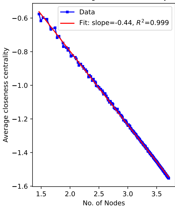
Log-Normal Fit and Plot of Nodes vs Average closeness centrality
