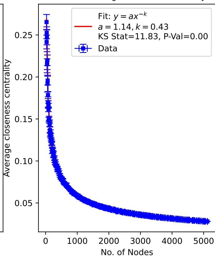
Power Law Fit and Plot of Nodes vs Average closeness centrality
