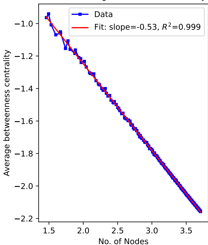
Log-Log Plot of Nodes vs Average betweenness centrality
