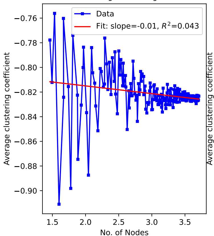
Log-Log Plot of Nodes vs Average clustering coefficient
